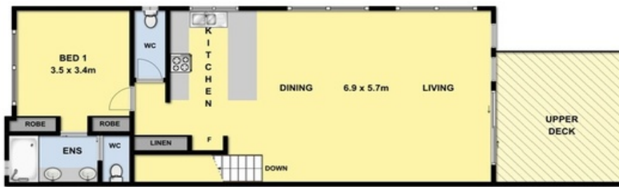
FIRST LEVEL
